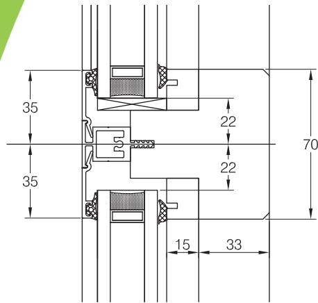
Alu-Timber Framing General arrangement showing Alu-Timber transom
