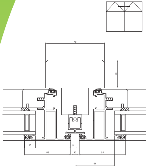
Alu-Timber Casement General arrangement showing opening vent
