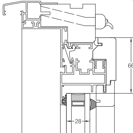
Alu-Timber Tilt & Turn General arrangement showing Alu-Timber head detail
