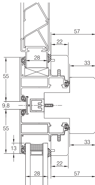
Alu-Timber Framing General arrangement showing Alu-Timber framing with opening vent
