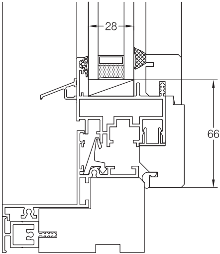
Alu-Timber Tilt & Turn General arrangement showing tilt & turn cill detail
