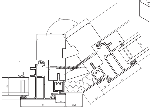
Alu-Timber Casement General arrangement showing 145 degree bay detail
