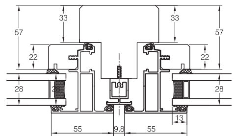
Alu-Timber Framing General arrangement showing Alu-Timber mullion with opening vent
