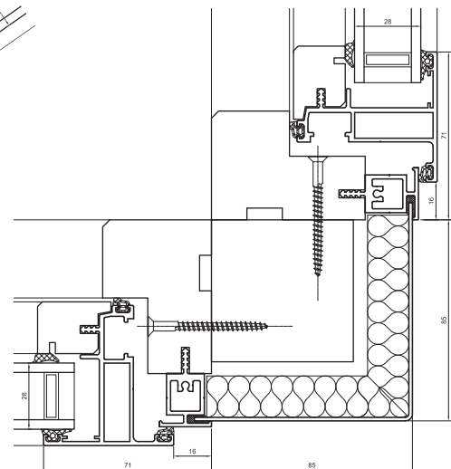
Alu-Timber Casement General arrangement showing external corner detail
