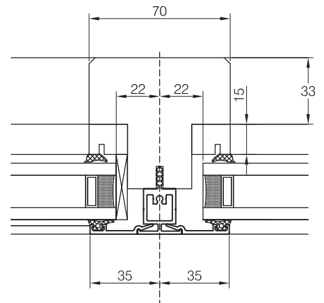
Alu-Timber Framing General arrangement showing mullion centres
