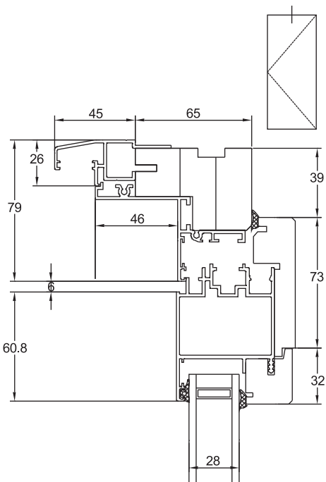
Alu-Timber Door General arrangement showing door head detail
