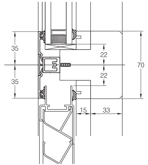
Alu-Timber Framing General arrangement showing Alu-Timber framing with fixed light and louvre
