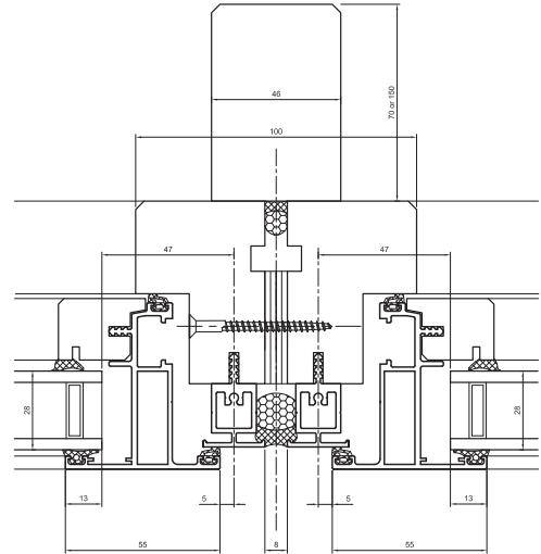
Alu-Timber Casement General arrangement showing Vent Coupled Windows with Mullion Combined Ix 1186.97 (70mm), Ix 4807.60cm (150mm)
