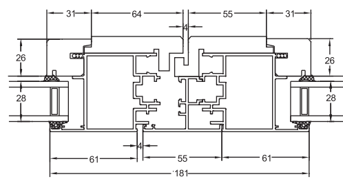
Alu-Timber Door General arrangement showing Alu-Timber open in double meeting stile
